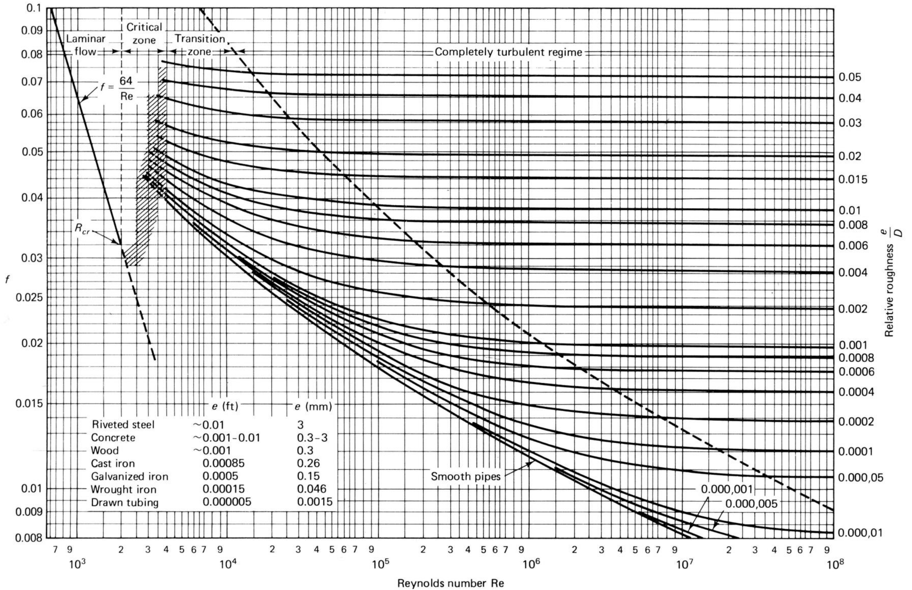
Moody diagram. (From L. F. Moody, Trans. ASME , Vol. 66, 1944.)
