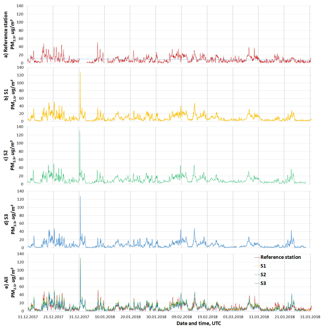
Figure 4. Results of PM 2.5 measurement from three SDS011 sensors and an official reference monitoring station in the period of 11 December 2017 to 31 March 2018: (a) Official reference station; (b) S1; (c) S2; (d) S3; (e) Comparison among the official reference station and three SDS011 sensors. 1 h averaged data was plotted.
